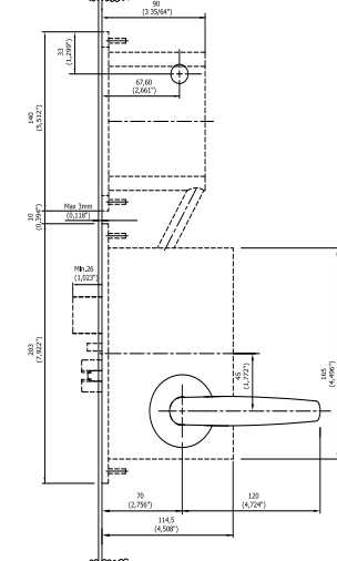
ELECTRONIC OVERRIDE ANSI DA lockcase without cylinder
