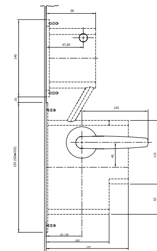
ELECTRONIC OVERRIDE EURO lockcase without cylinder
