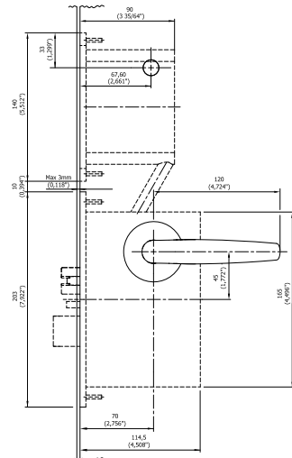
ELECTRONIC OVERRIDE ANSI DB lockcase without cylinder
